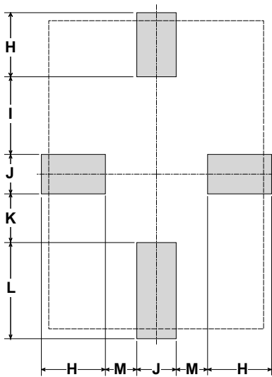
PCB Footprint
