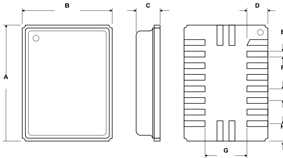
SM-20H Package Drawing
